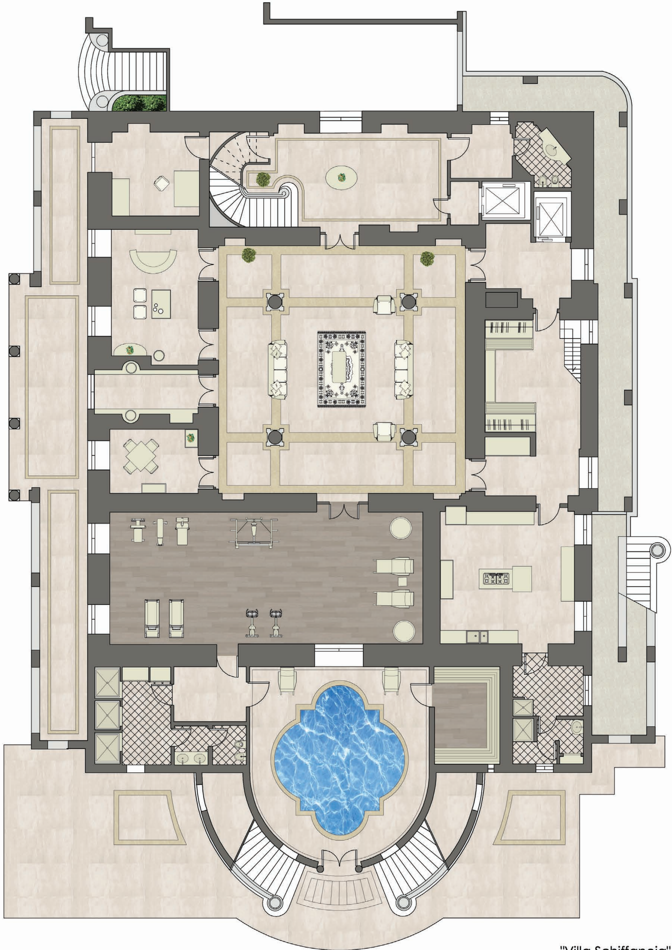
"Villa Schiffanoia" GROUND FLOOR
